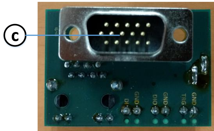
Figure 1-2: Argos3D-P22x break-out board backside view
