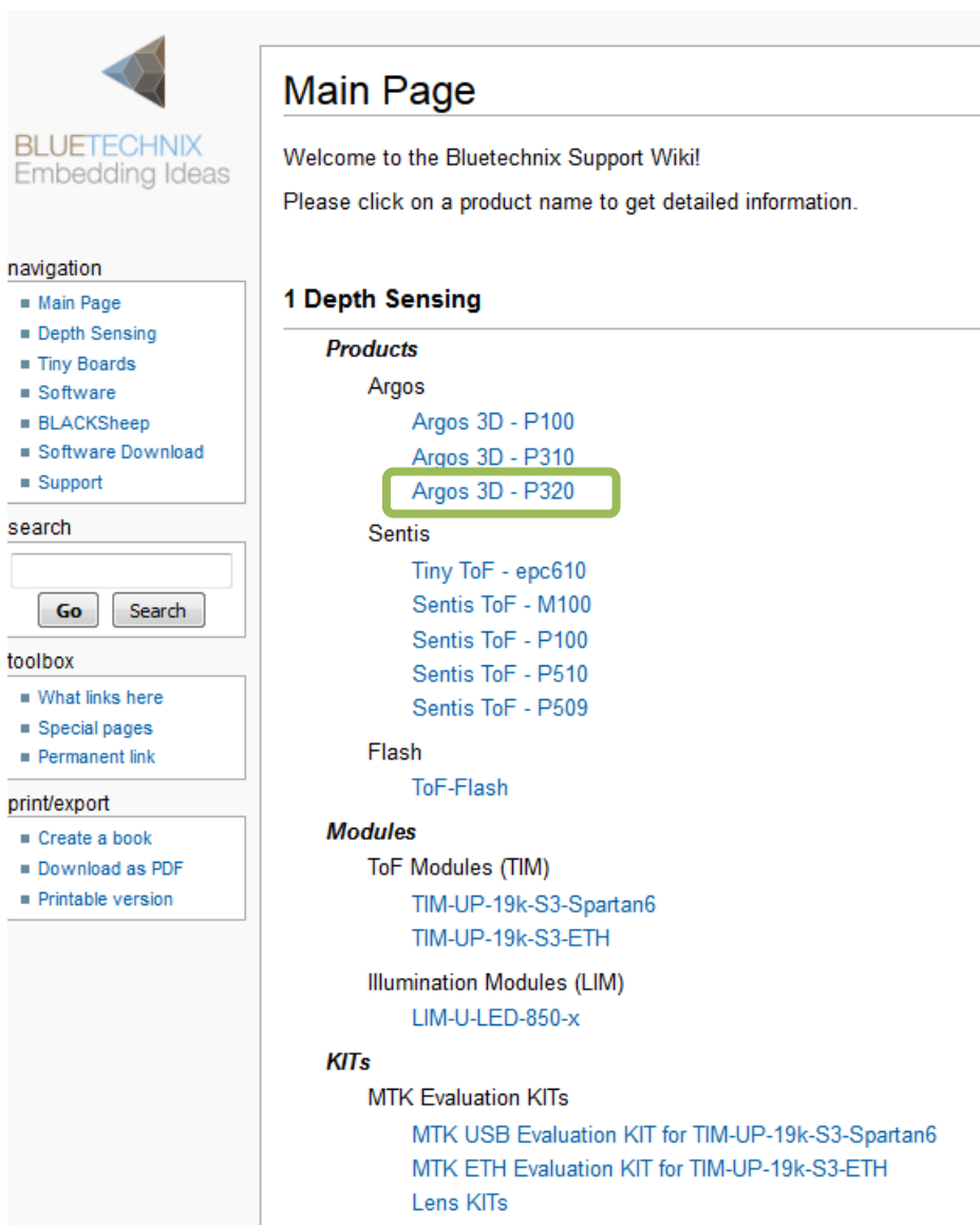
Figure 2-2: Start-up screen
