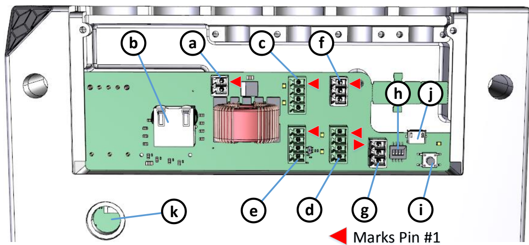
Figure 1-2: Argos3D–P32X connectors and interfaces
