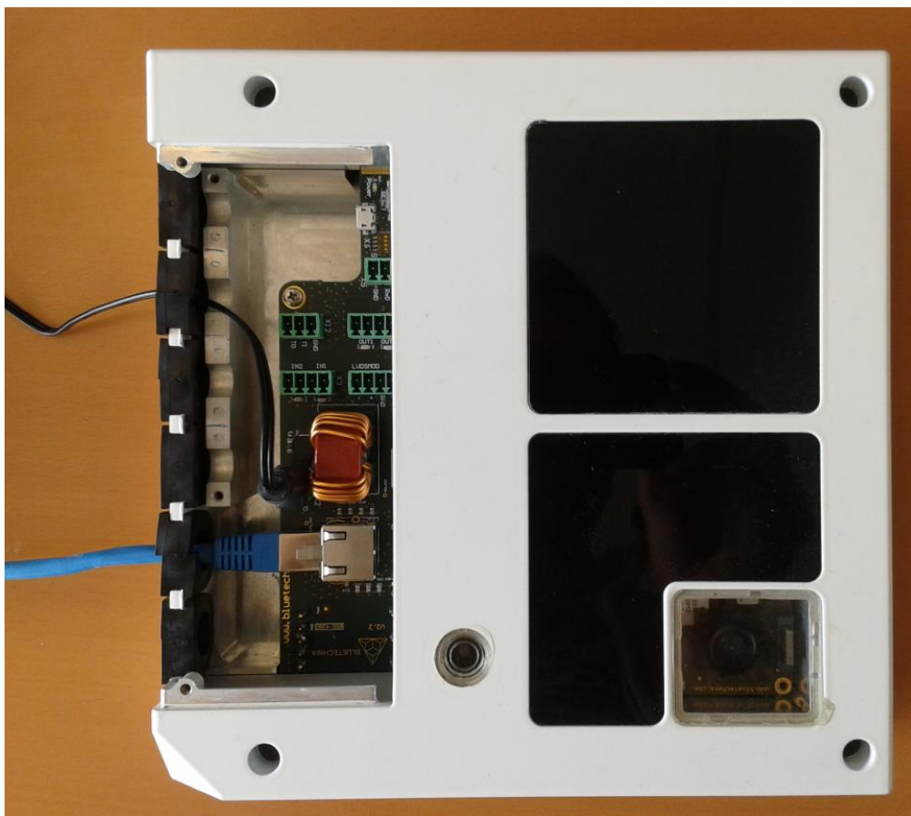
Figure 1-3: Argos3D–P32X with connected power supply and Ethernet cable
