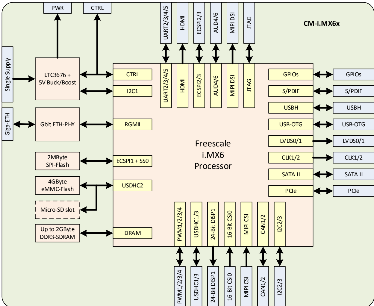
Figure 2-1 Detailed block diagram of the CM-i.MX6x
