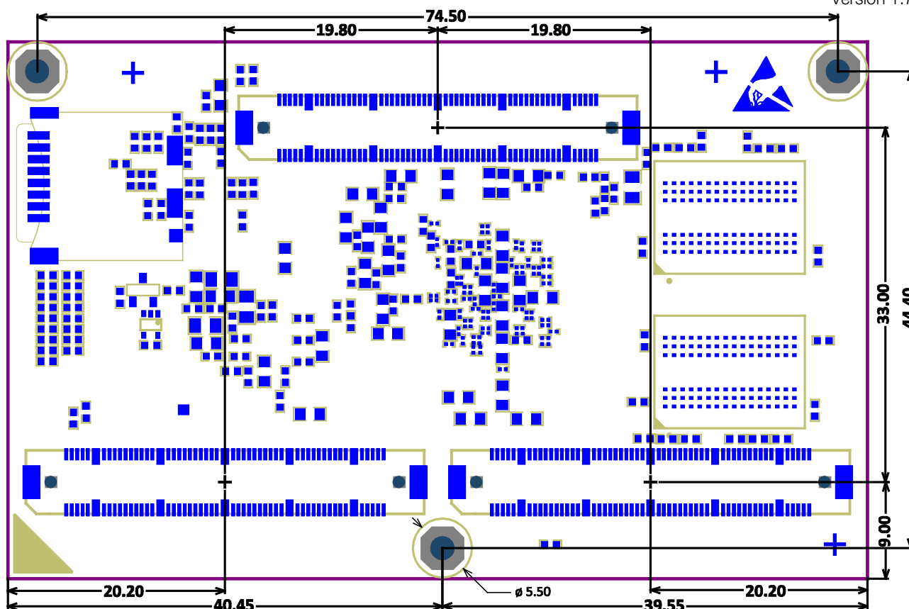
Figure 6-2 Mechanical outline (bottom view)
