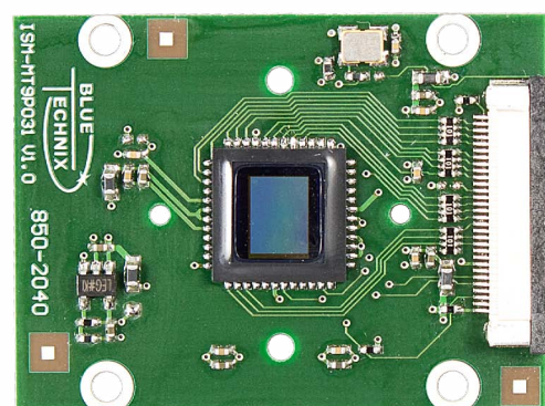
ISM-MT9P031-Color
